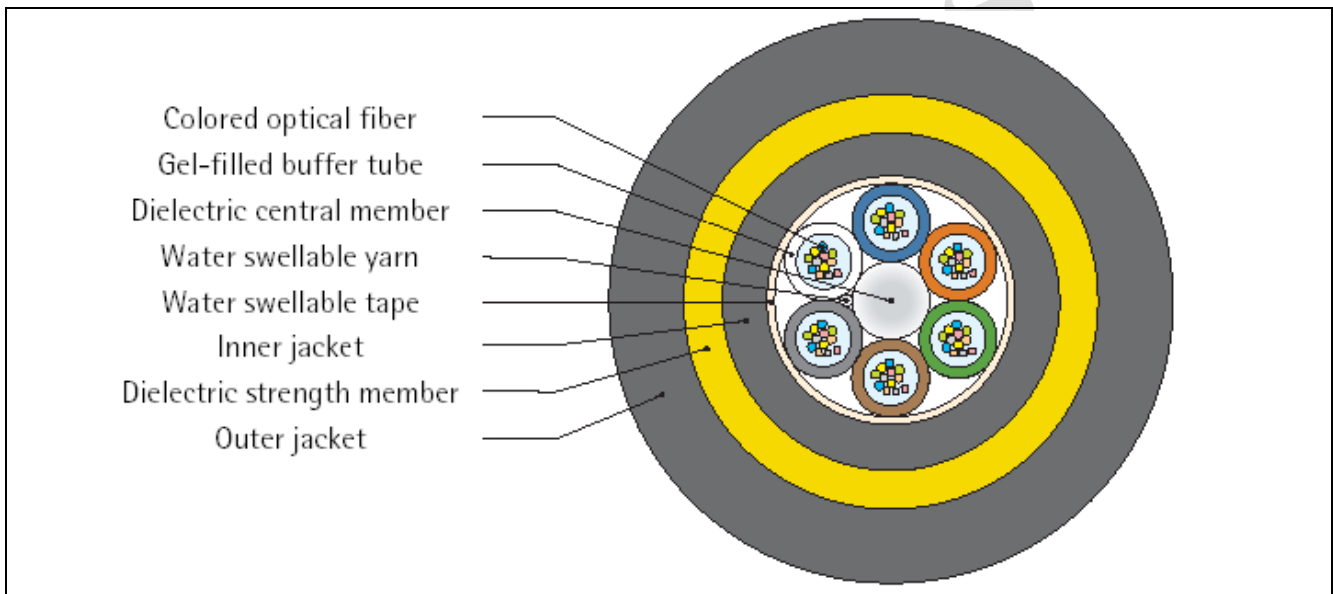
All-Dielectric Self Supporting Optic Fiber Cable Components
