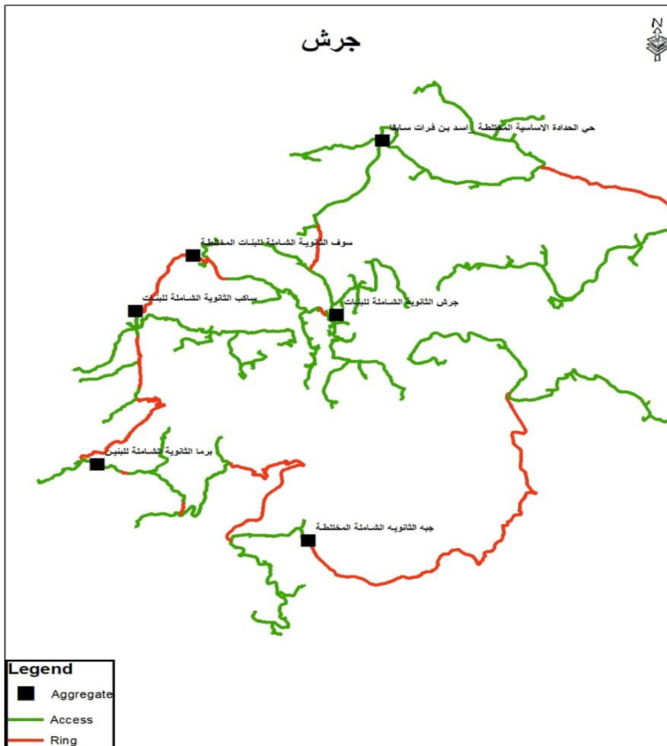
Figure 3: Fiber Route – Jarash
