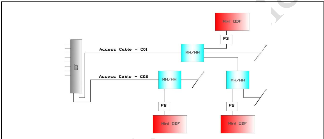
Figure 6: Connection between Aggregate Point to the Entities - Access Network
