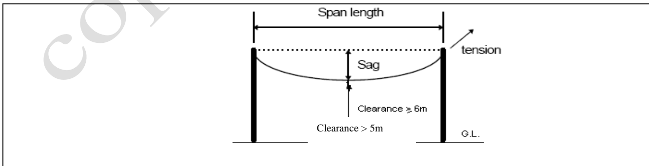
Aerial Cable Sag and Clearance
