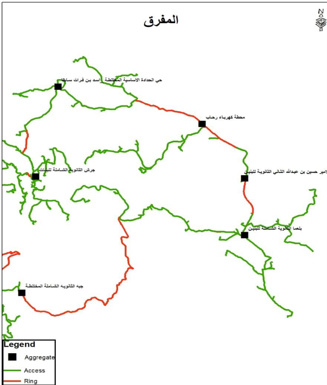
Figure 5: Fiber Route – Mafraq
