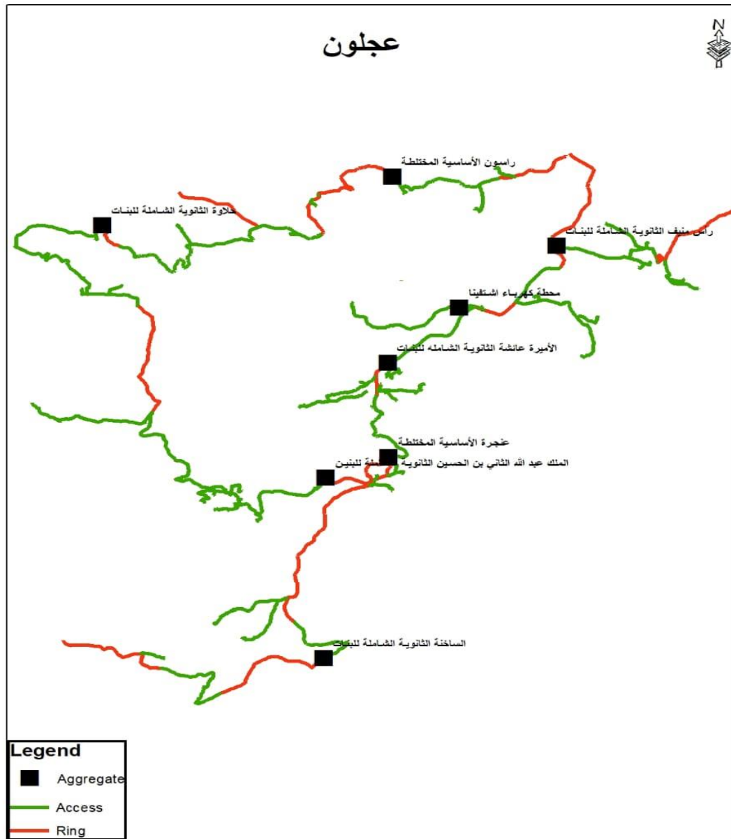
Figure 4: Fiber Route – Ajloun
