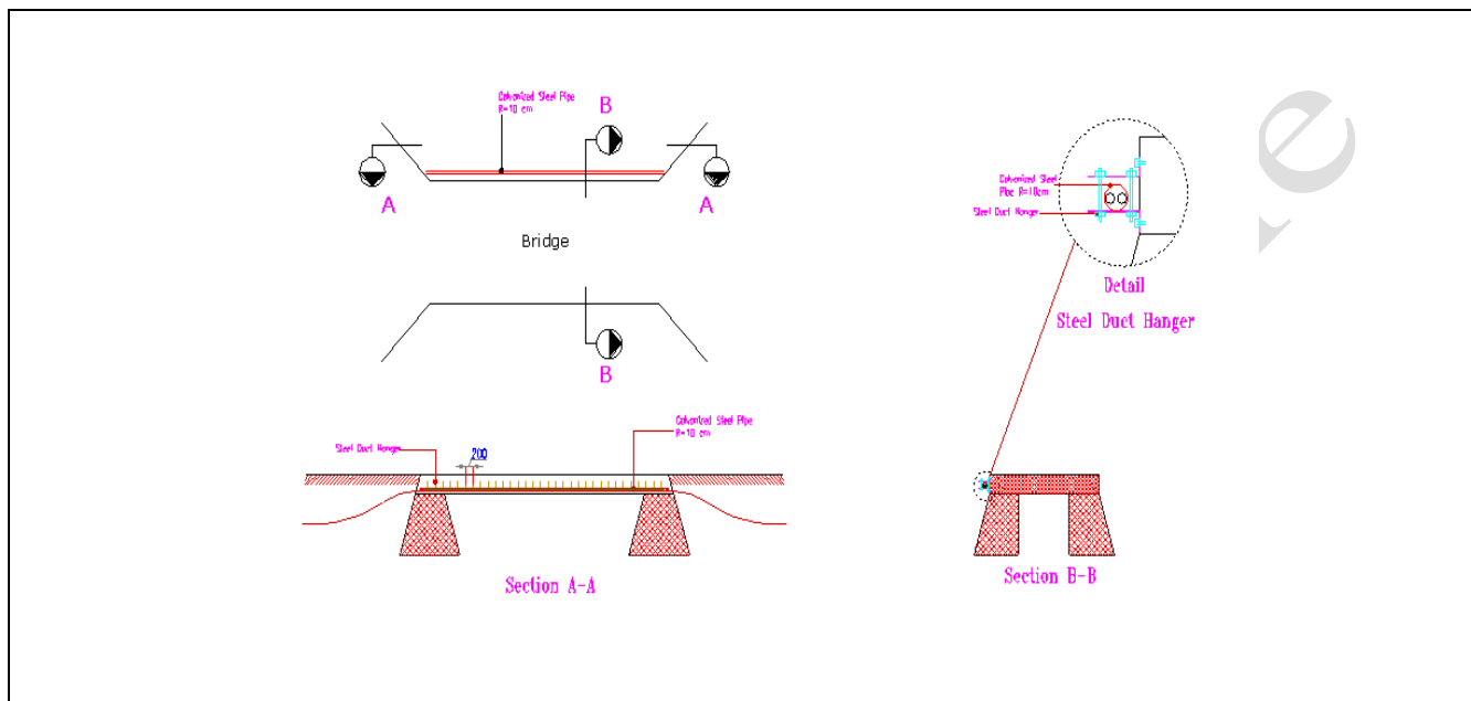
Bridge Crossing Details
