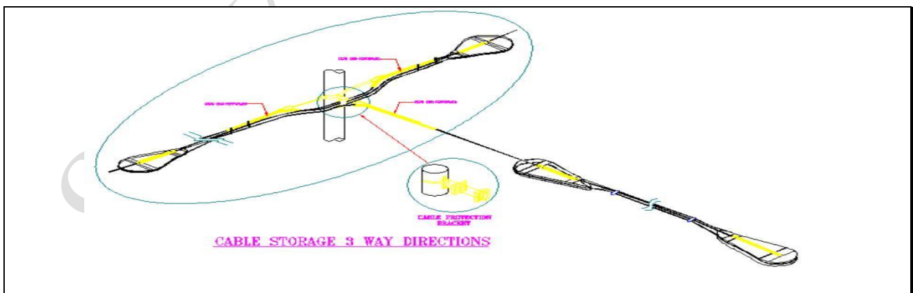
Figure_8 - Aerial Cable Storage Configuration for Angled Cables
