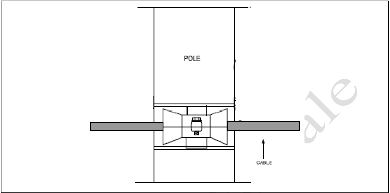
Pass-Through Bracket
