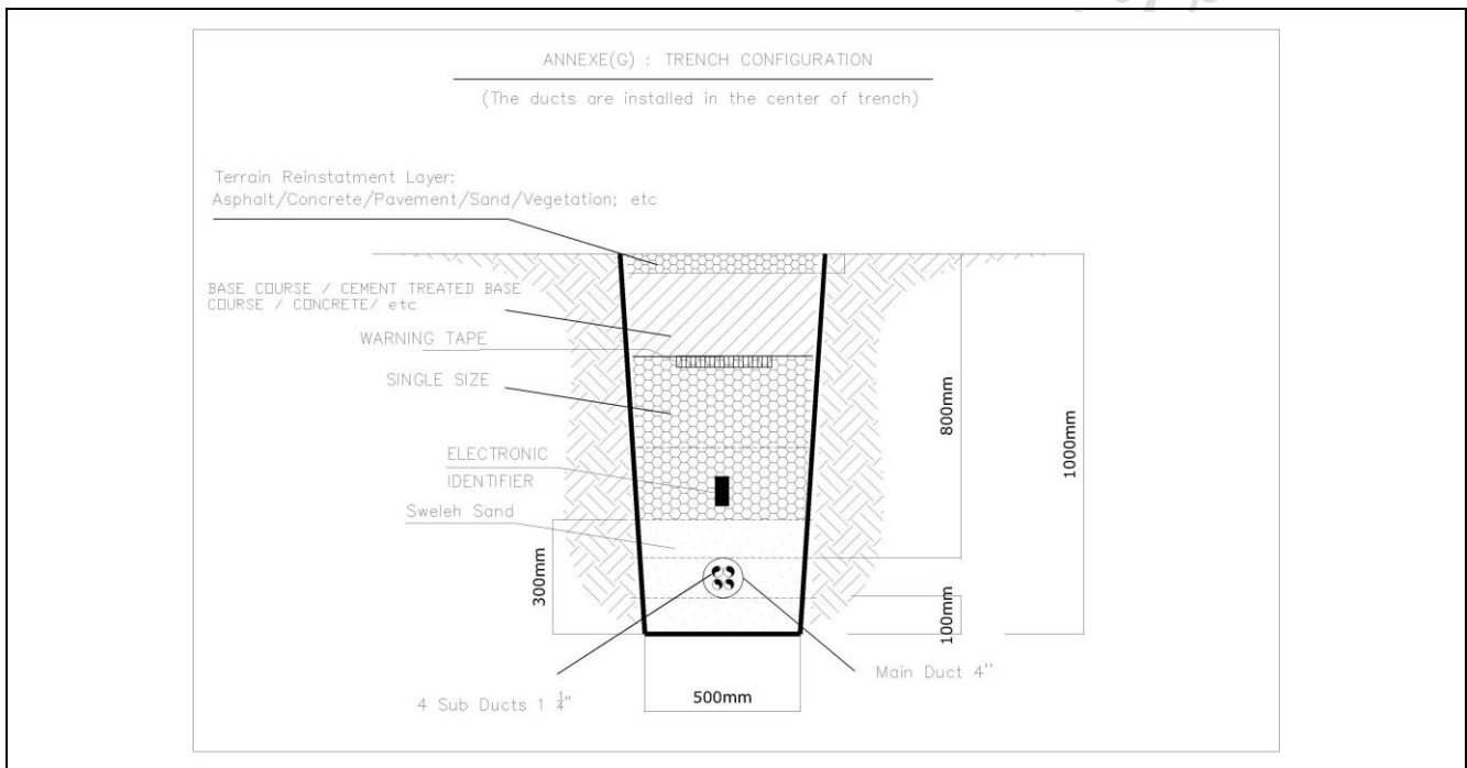
Trench Specifications for Four ducts inside one main duct
