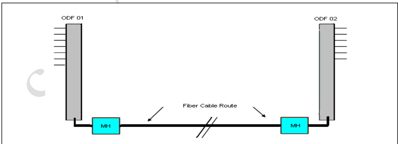
Figure 7: Connection between Aggregate Point to Aggregate Point - Ring Network
